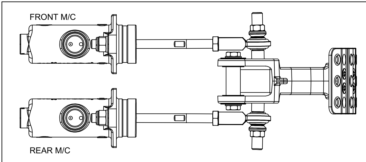
Figure 2. Initial Balance Bar Lever Adjustment
