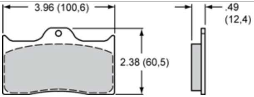
Wilwood Brake Pad Plate #7112
